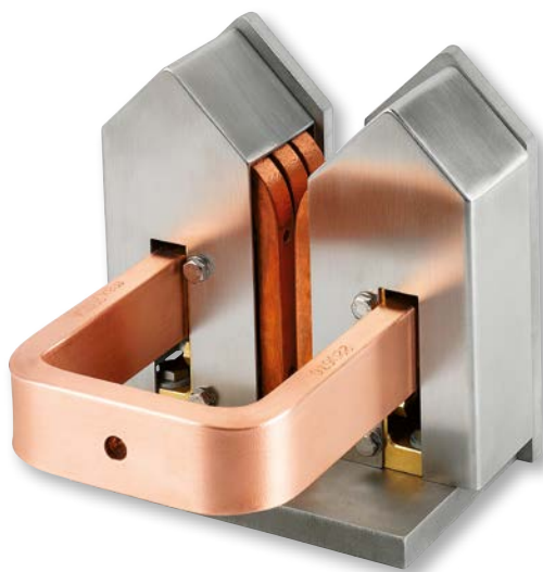
Contact saddle in special design with current feed through a bracket
