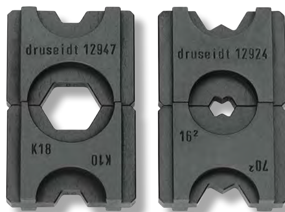
die-sets for crimping head Part-No. 14242 druseidt system dies size I flat design
