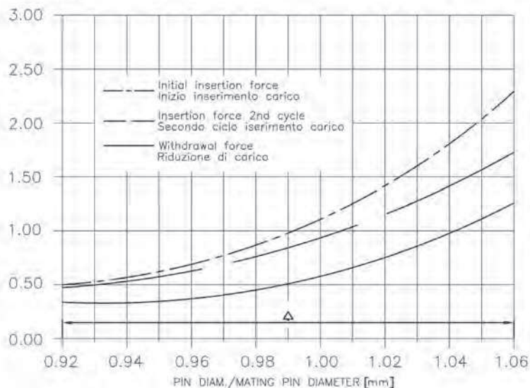
CARICO/FORCE [N]
