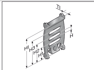
Separator, open
