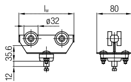
Cable Trolley
