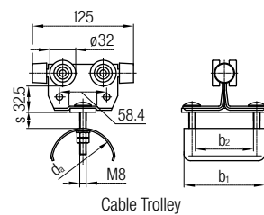
Cable Trolley
