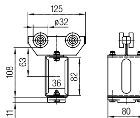
Towing Trolley
