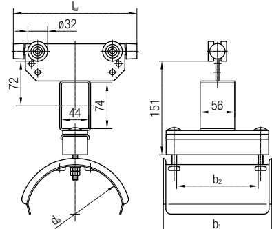
Towing Trolley
