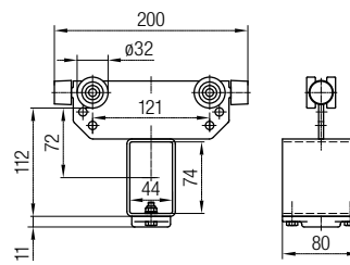
Towing Trolley
