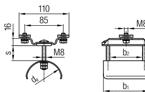
End Clamp
